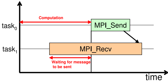
Fig. 6. Late-Sender pattern
