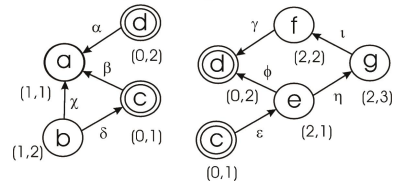
Fig 3.2 Complementary graphs
