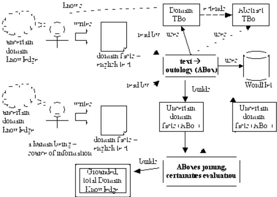
Fig. 1. Solution concept
