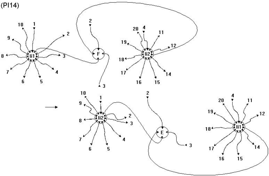
Fig. 8. Graph grammar production allowing for breaking an element edge, for the edge surrounded by two broken interiors
