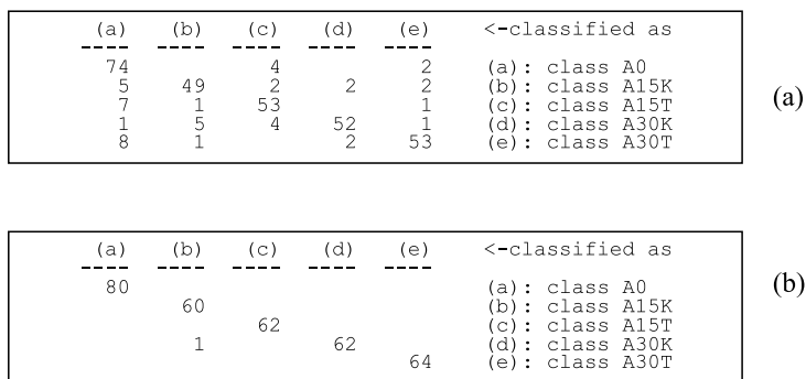
Fig. 1. Confusion matrices obtained on the same dataset with program See5: (a) – default settings, (b) – after selecting the option: Boost (10 trials)
