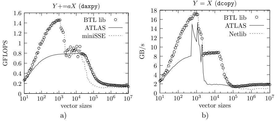
Fig. 2. Performance data for the daxpy (a) and dcopy (b) operations using the generated, optimal BLAS interface (BTL lib). The threshold values and the best implementations available are determined automatically.
