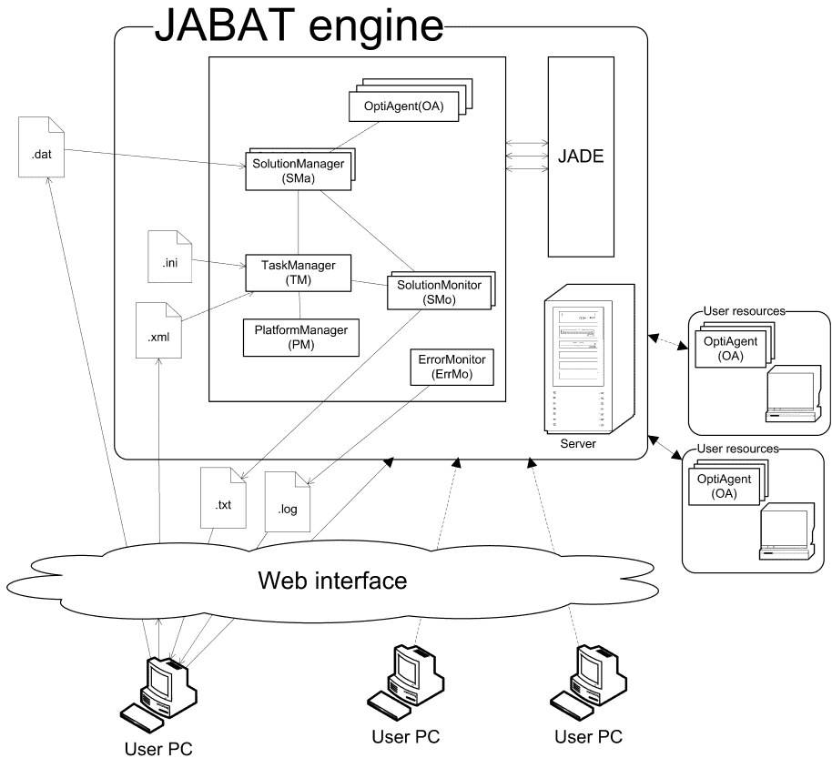
Fig. 3. e-JABAT architecture
