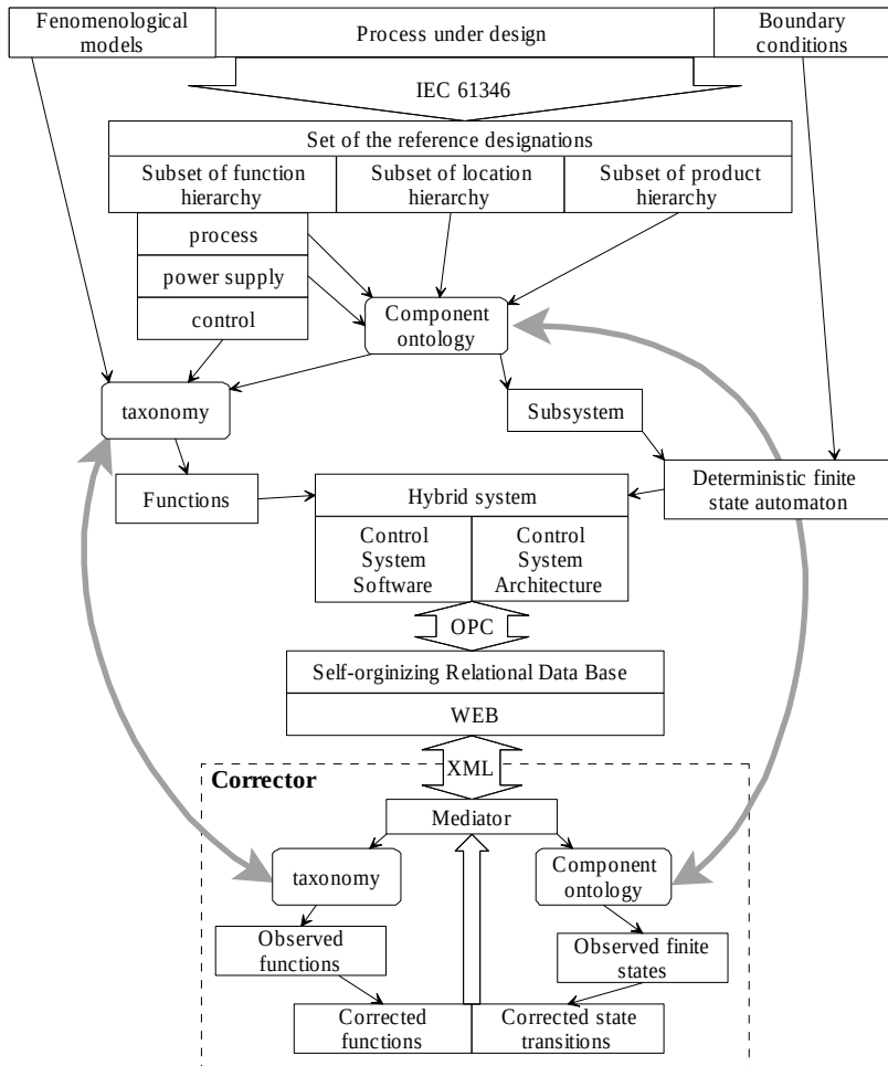
Fig. 2. System architecture
