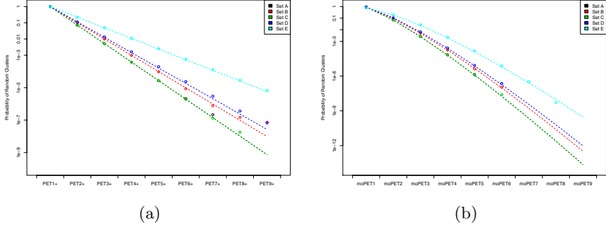
Fig. 3. Comparing simulation and analytical results. Probability of a random (A) PETn+ or (B) moPETn cluster produced by chance, as estimated by Monte Carlo simulations (points) and computed analytically (dashed lines).
